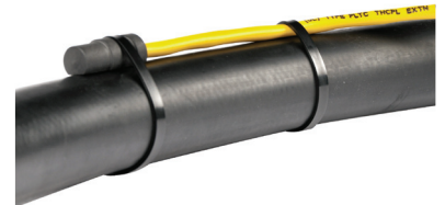
Exertherm Cable Sensor
